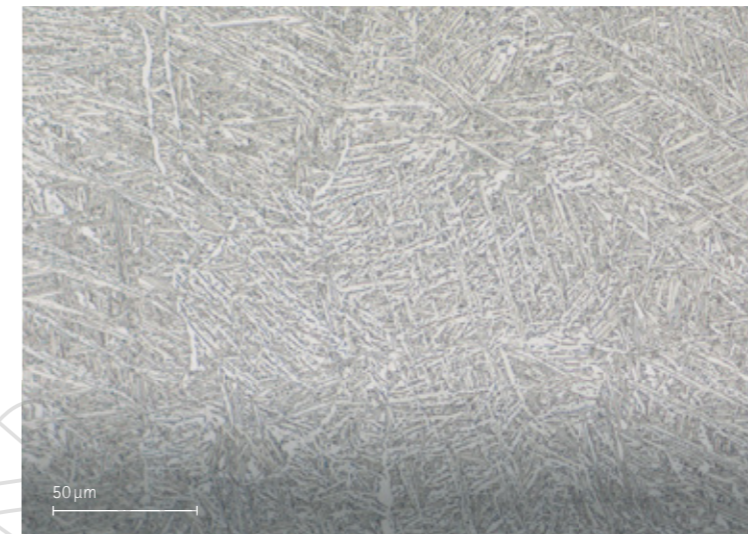
Heat treated microstructure. Etched according to ASTM E407 modified recipe #190.
